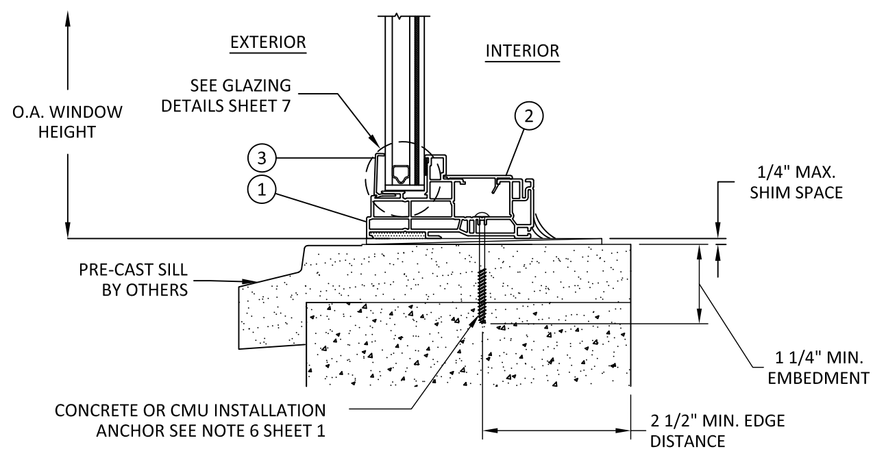
D 3 VERTICAL SECTION PRE-CAST SILL - CONCRETE/MASONRY THROUGH FRAME INSTALLATION (REPLACEMENT)
