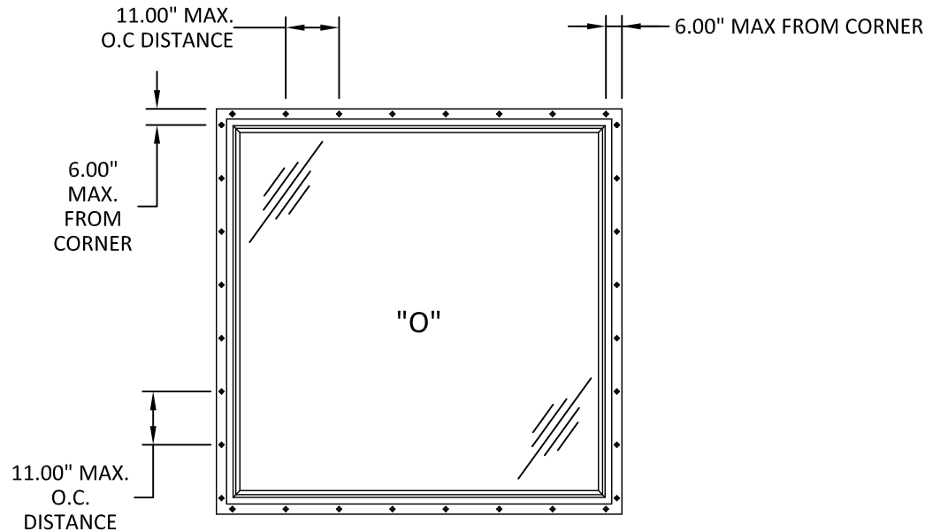
ANCHOR LAYOUT NAIL FIN INSTALLATION
