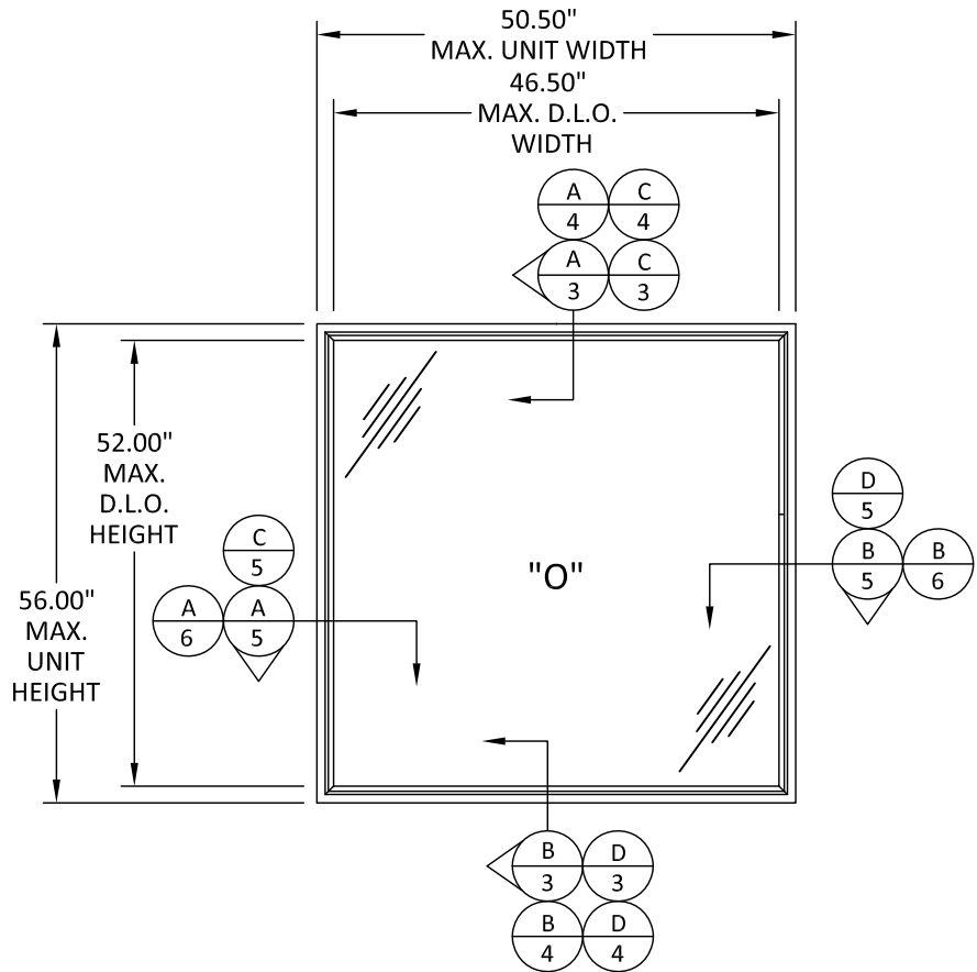
ELEVATION FIXED WINDOW
