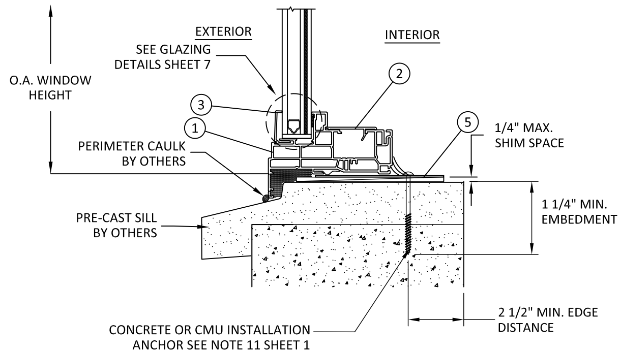
B 3 VERTICAL SECTION PRE-CAST SILL - CONCRETE/MASONRY CLIP INSTALLATION
