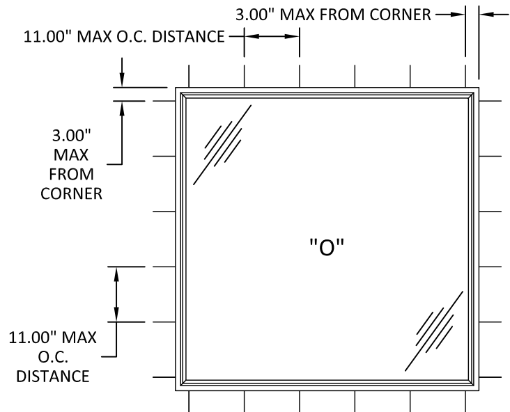
ANCHOR LAYOUT THROUGH FRAME/CLIP INSTALLATION
