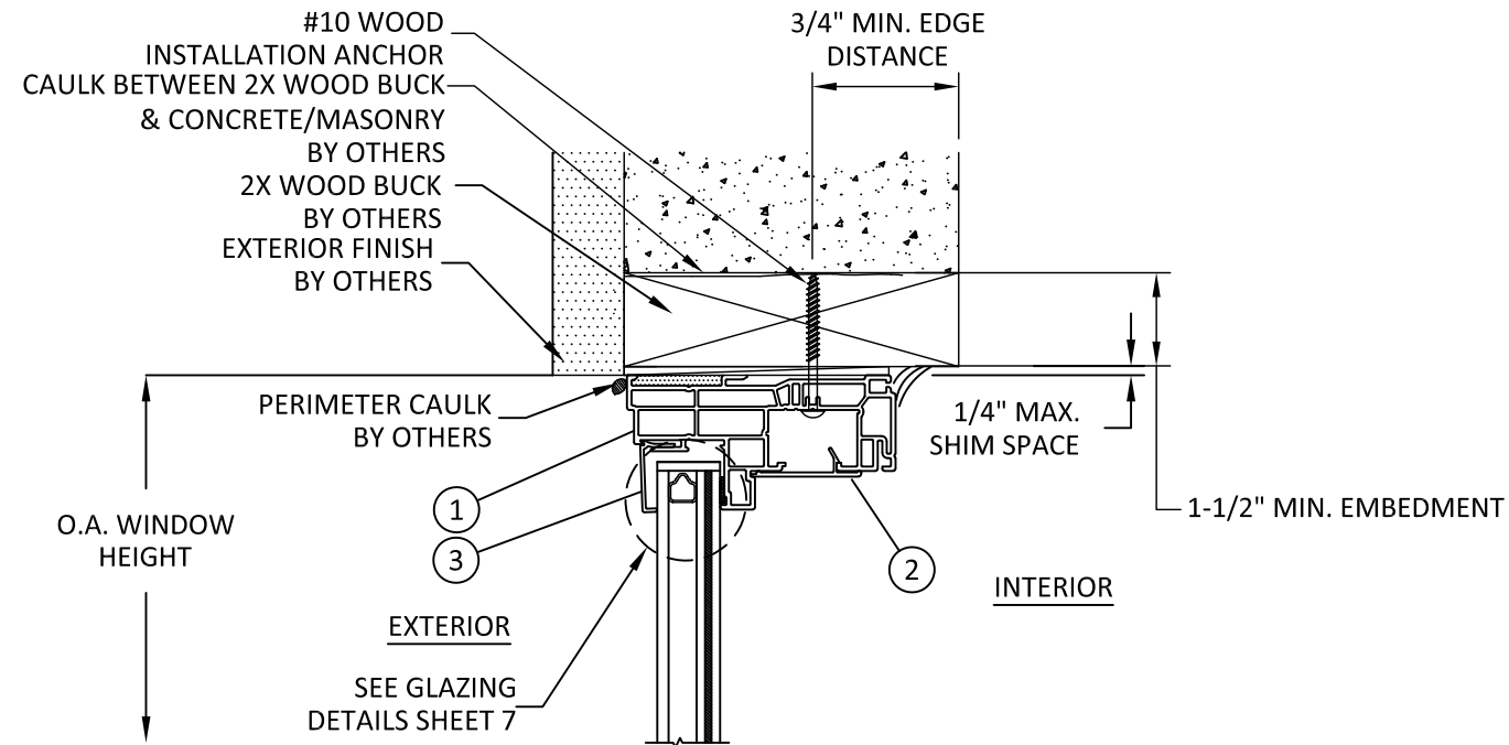
A 3 VERTICAL SECTION HEAD - 2X WOOD BUCK THROUGH FRAME INSTALLATION (REPLACEMENT)
